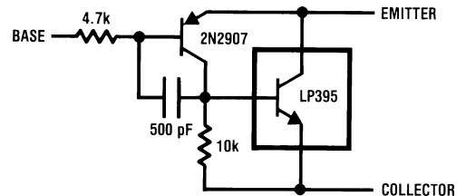
Composite PNP
